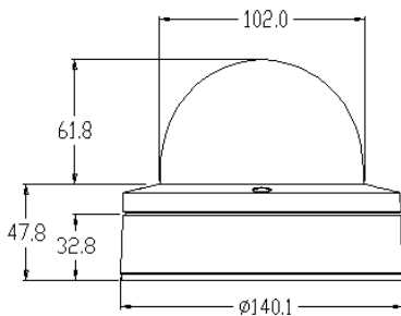
Figure 7.2 Side view
